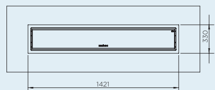
CEILING RECESS FRAME 4500W
